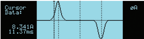
Acquired Current waveform (iX Display).
