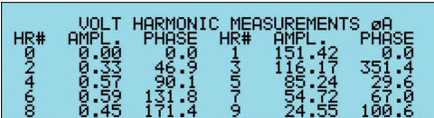
Voltage harmonic measurement table display in absolute values (iX Display).
