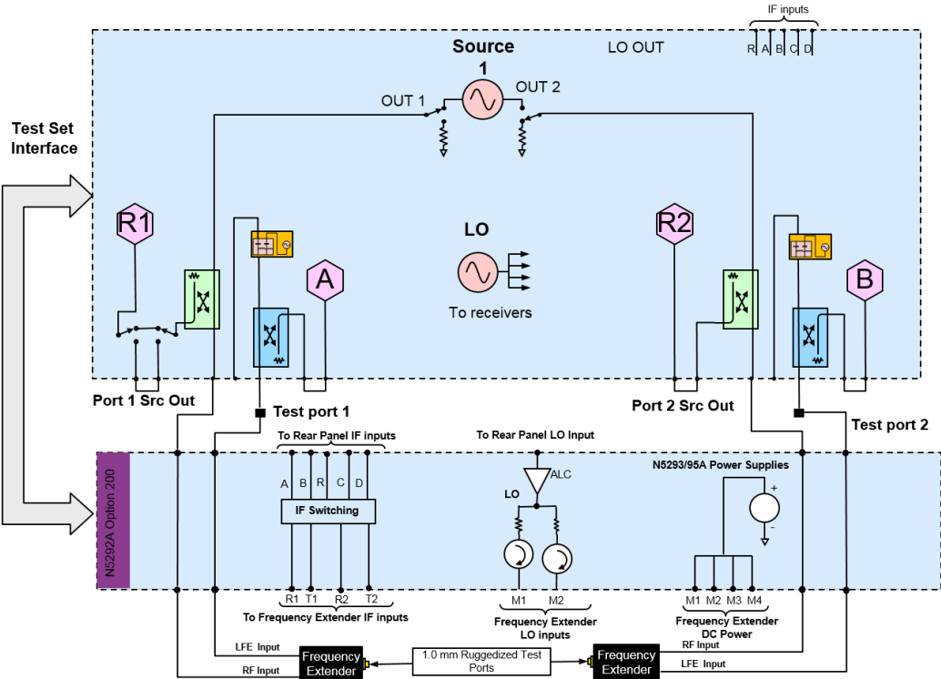
N5290/91A Option 201 System level block diagram (N5222B with Option 205)
