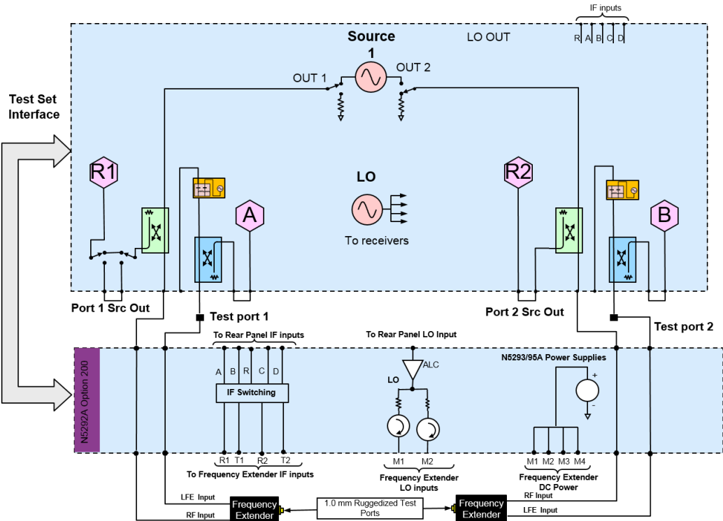
N5290/91A Option 202 System level block diagram (N5227B with Option 205)
