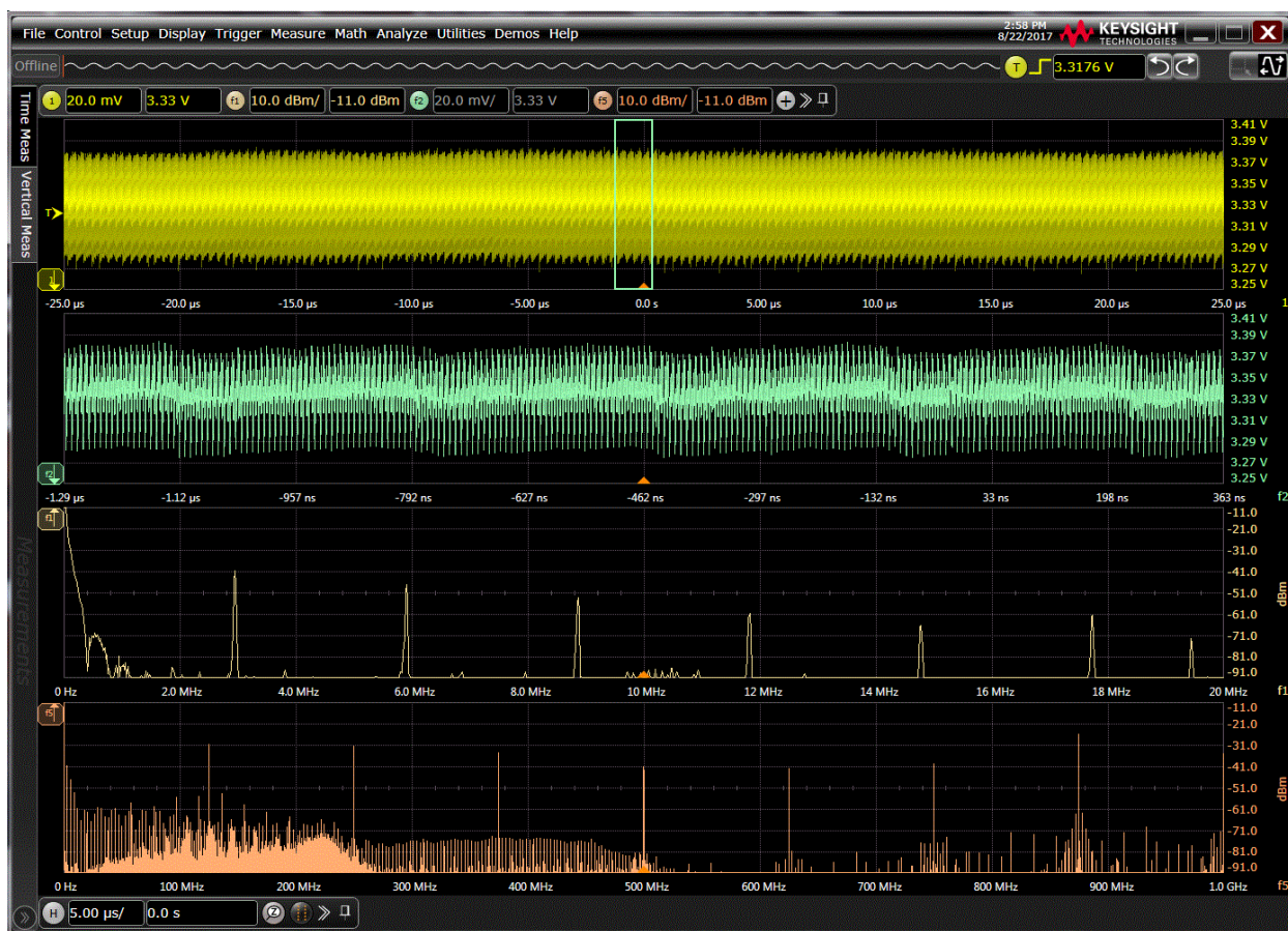
Figure 22. N7020A Power Rail Probe and S-Series High-definition oscilloscope measuring the noise on a 3.3 V supply.
