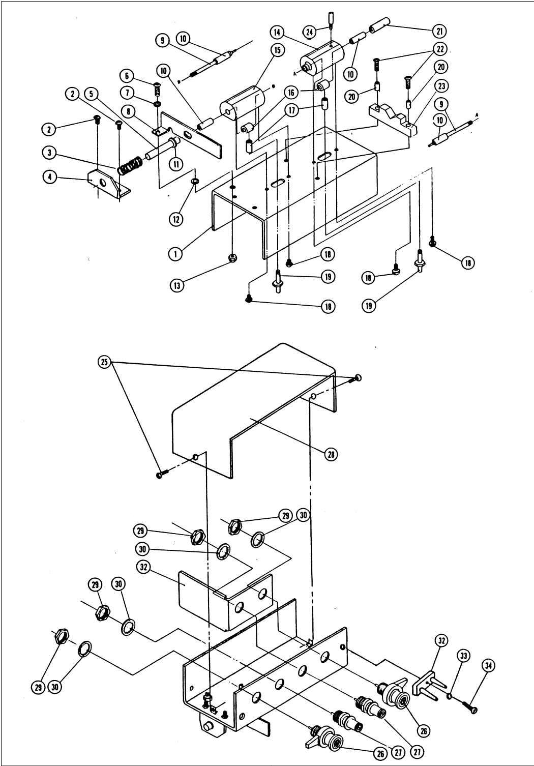
Figure 2-1 Parts Identification
