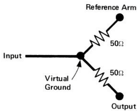
Figure 3 Keysight 11667B schematic
