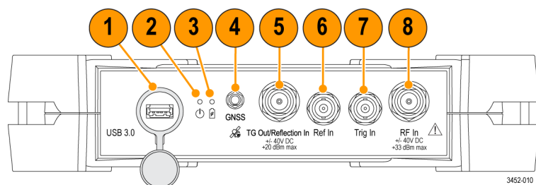
Figure 1: Front panel
