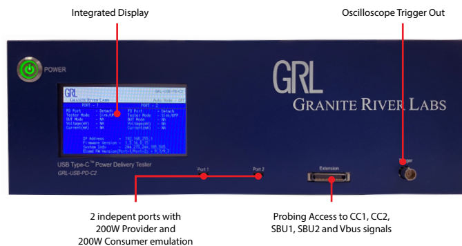
Front Panel
