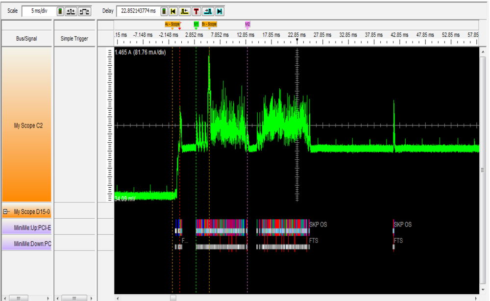
Figure 14. The data from the oscilloscope is display on the same time scale to show the exact voltage, current, and power consumption of the device.
