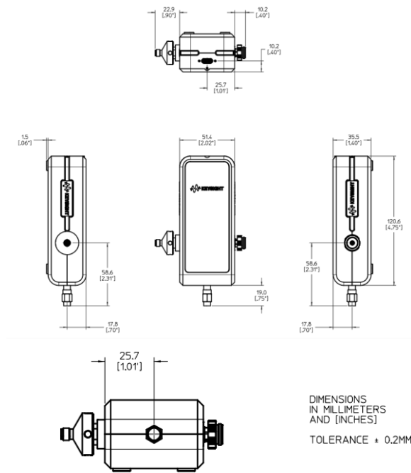
Mechanical dimension for U9391M
