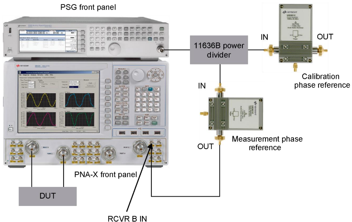
Figure 1. NVNA setup for arbitrary frequency grid (U9391C/F/G)
