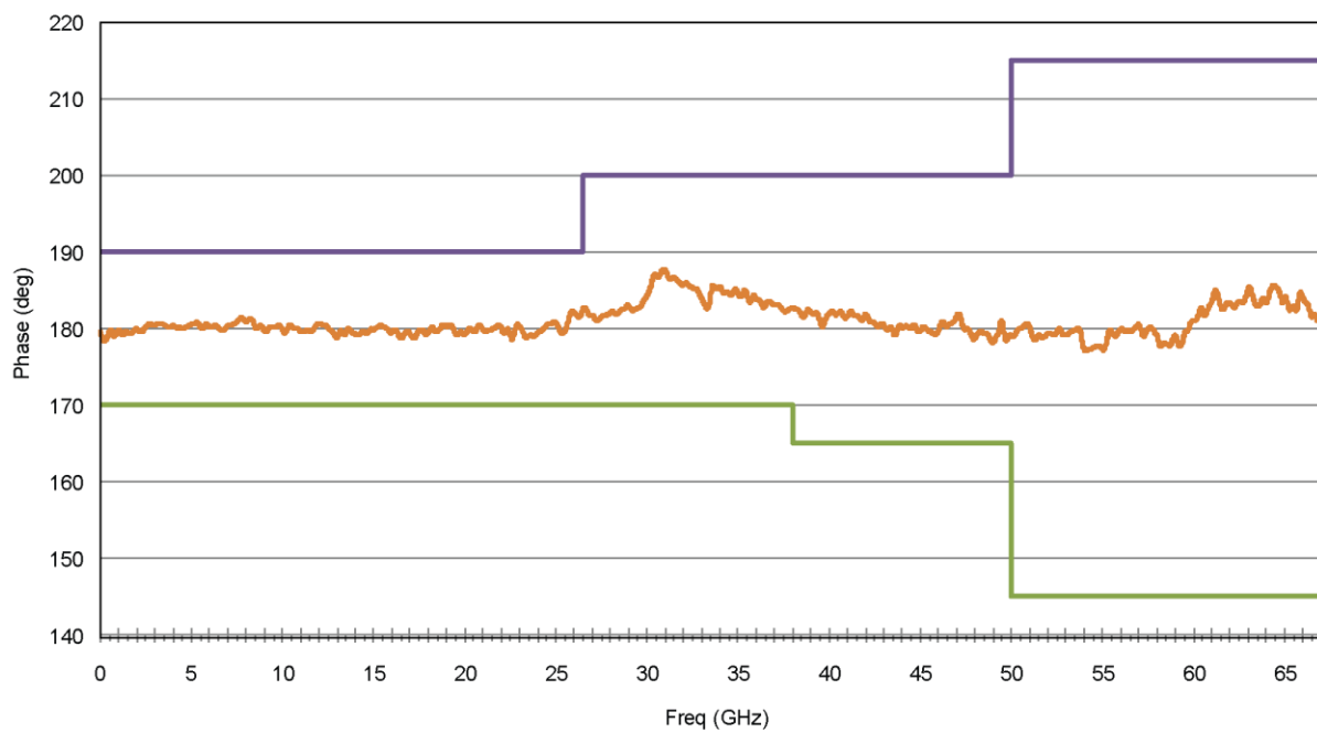
Figure 7. U9391G Comb Generator Phase at 10 MHz PRF
