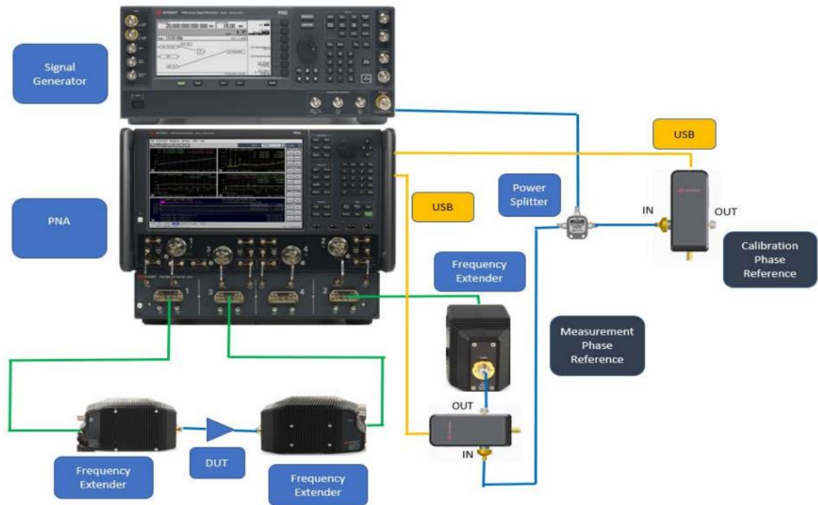
Figure 2. NVNA setup for arbitrary frequency grid (U9391M)
