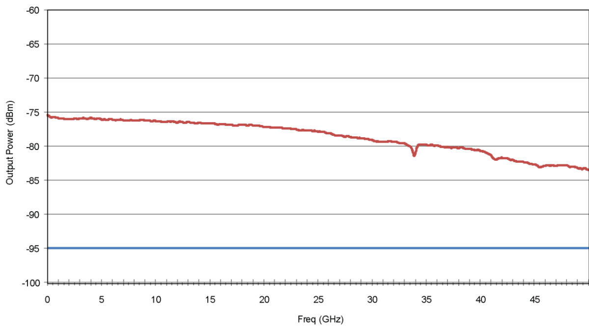
Figure 9. U9391F Comb Generator Output Power at 10 MHz PRF
