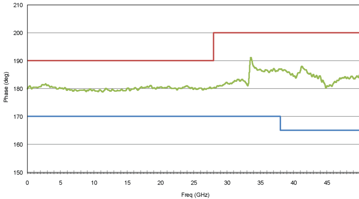
Figure 6. U9391F Comb Generator Phase at 10 MHz PRF
