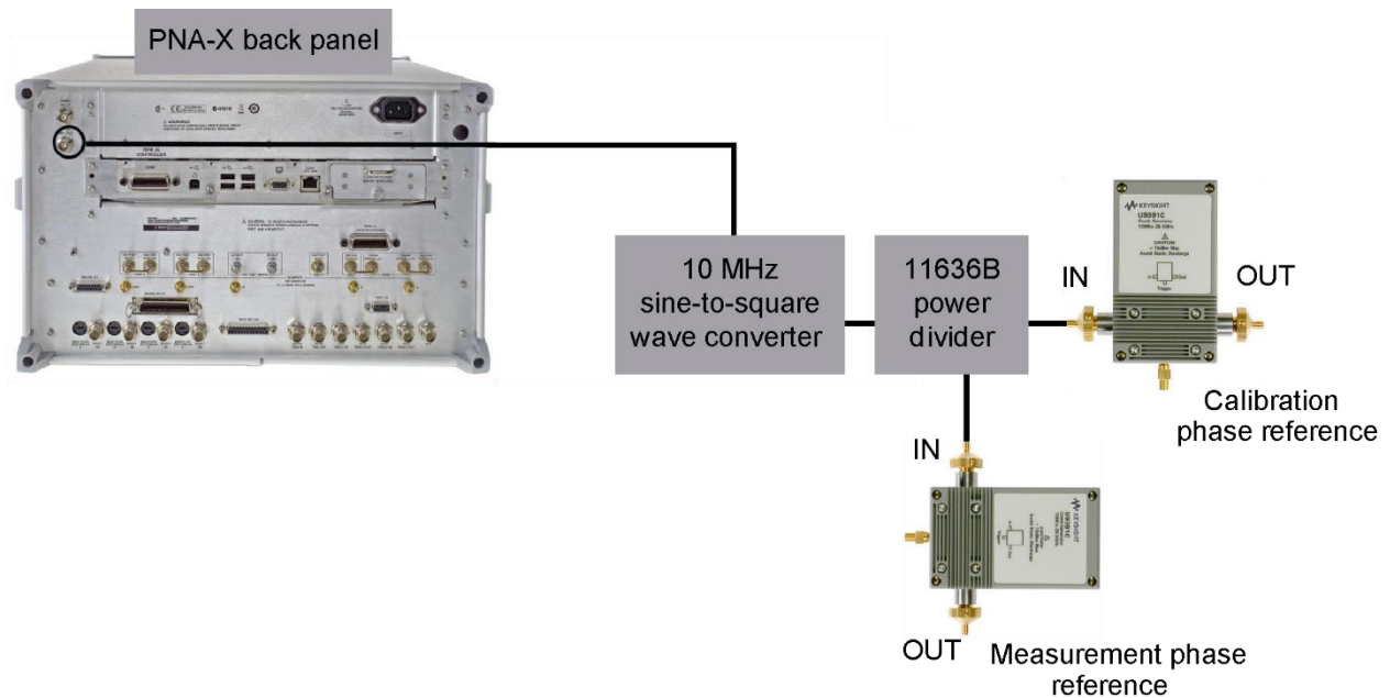
Figure 3. Measurement with sine-to-square wave converter (only for U9391C/F/G)
