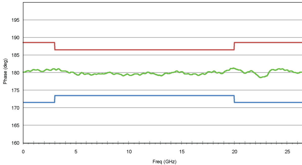
Figure 5. U9391C Comb Generator Phase at 10 MHz PRF
