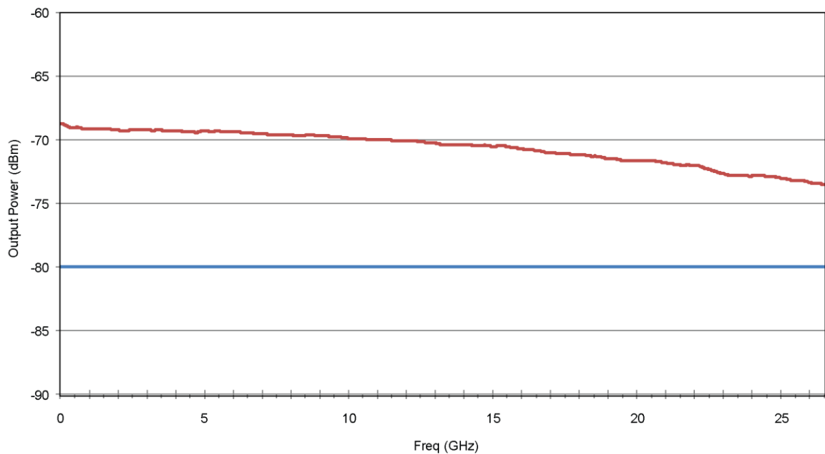
Figure 8. U9391C Comb Generator Output Power at 10 MHz PRF
