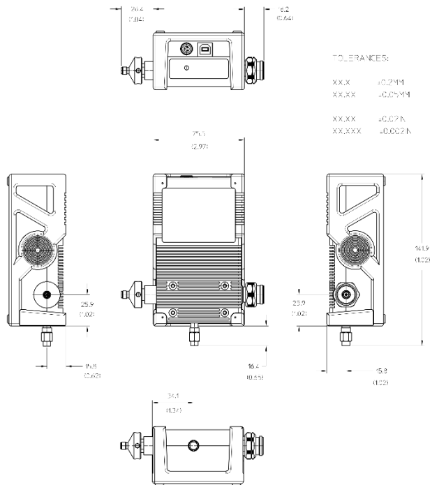
Mechanical dimension for U9391G
