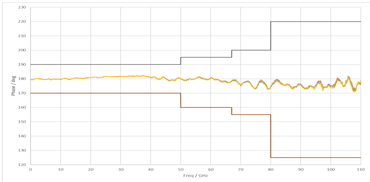
Figure 11. U9391M Comb Generator Phase at 10 MHz PRF
