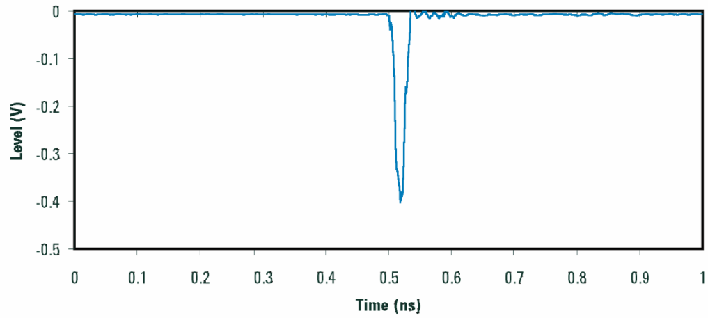
Figure 4. U9391C/F pulse
