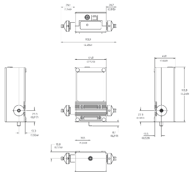
Mechanical dimension for U9391F
