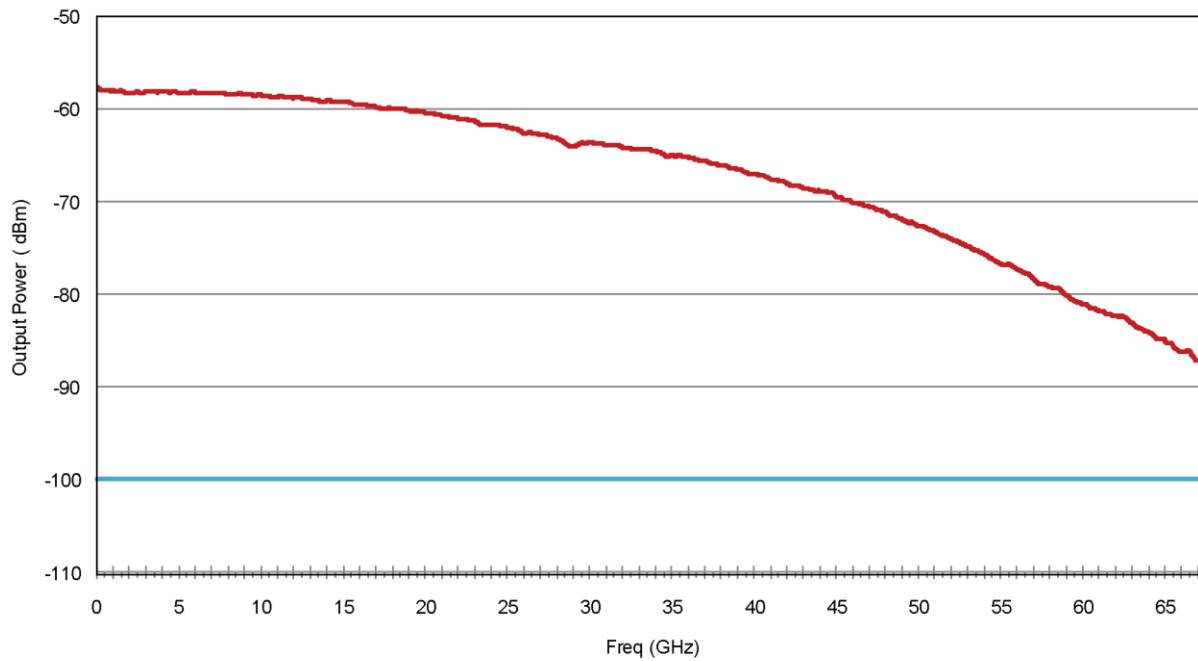
Figure 10. U9391G Comb Generator Output Power at 10 MHz PRF
