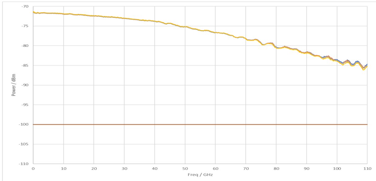
Figure 12. U9391M Comb Generator Output Power at 10 MHz PRF
