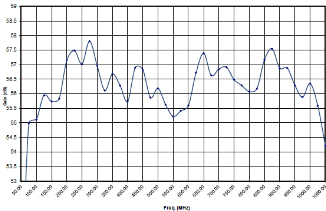
TYPICAL SMALL SIGNAL GAIN @ -20 dBm INPUT
