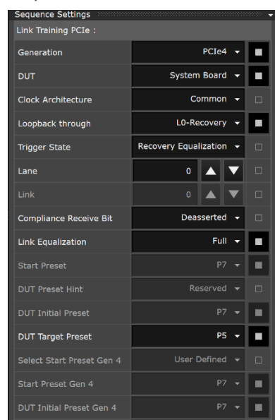
Figure 14. The interactive link training capability of J-BERT M8020A significantly reduces the effort to generate and tune a loopback sequence for your device under test. The example shows the properties you can choose for the PCIe 8 GT/s or 16 GT/s link training state machine.
