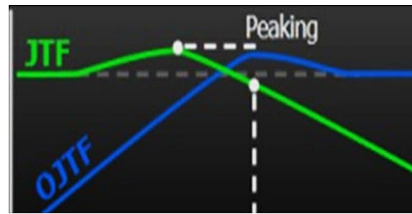
Figure 26. Each M8041A/51A analyzer has a built-in clock recovery. Choose between first and second order PLL.
