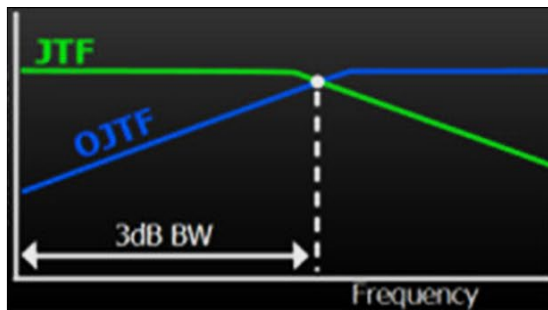
Figure 26. Each M8041A/51A analyzer has a built-in clock recovery. Choose between first and second order PLL.
