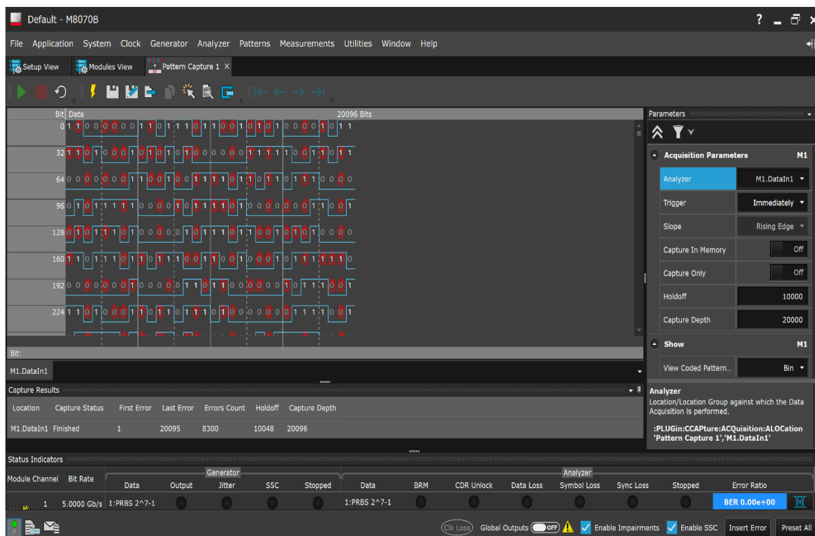
Figure 24. The J-BERT M8020A analyzer can capture up to 2 Gbit per channel. Capture events and depth can be defined. The captured pattern can be exported and loaded as generator pattern or as expected pattern for further error analysis. The example shows errored bits in red with navigation arrows.
