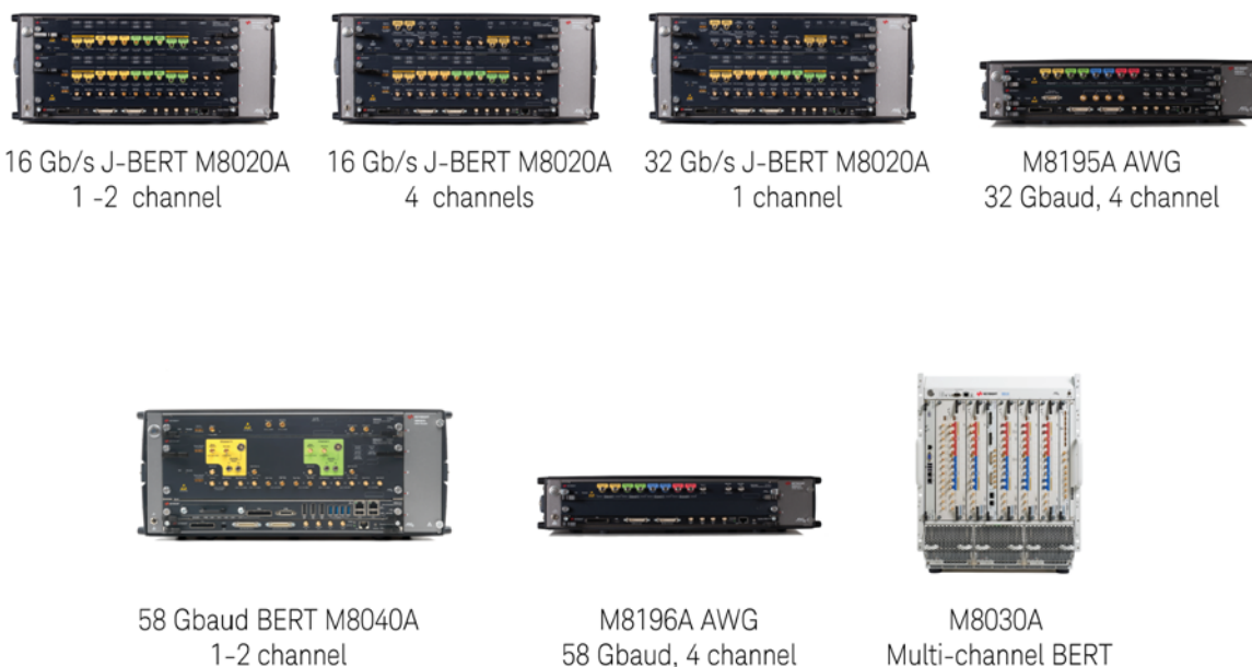
Figure 1 The M8000 Series BER Test Solution is highly integrated and scalable to address the test challenges of the next generation of high-speed digital receiver test.
