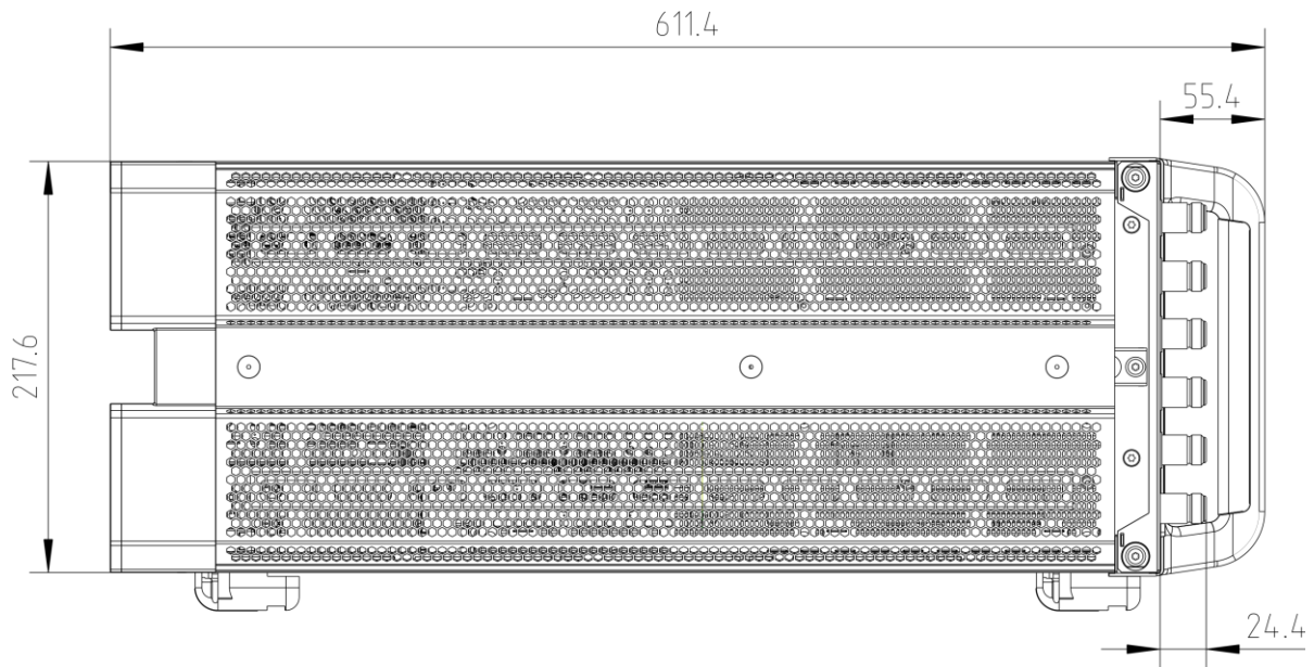
Side view of the R&S®ZNB T8
