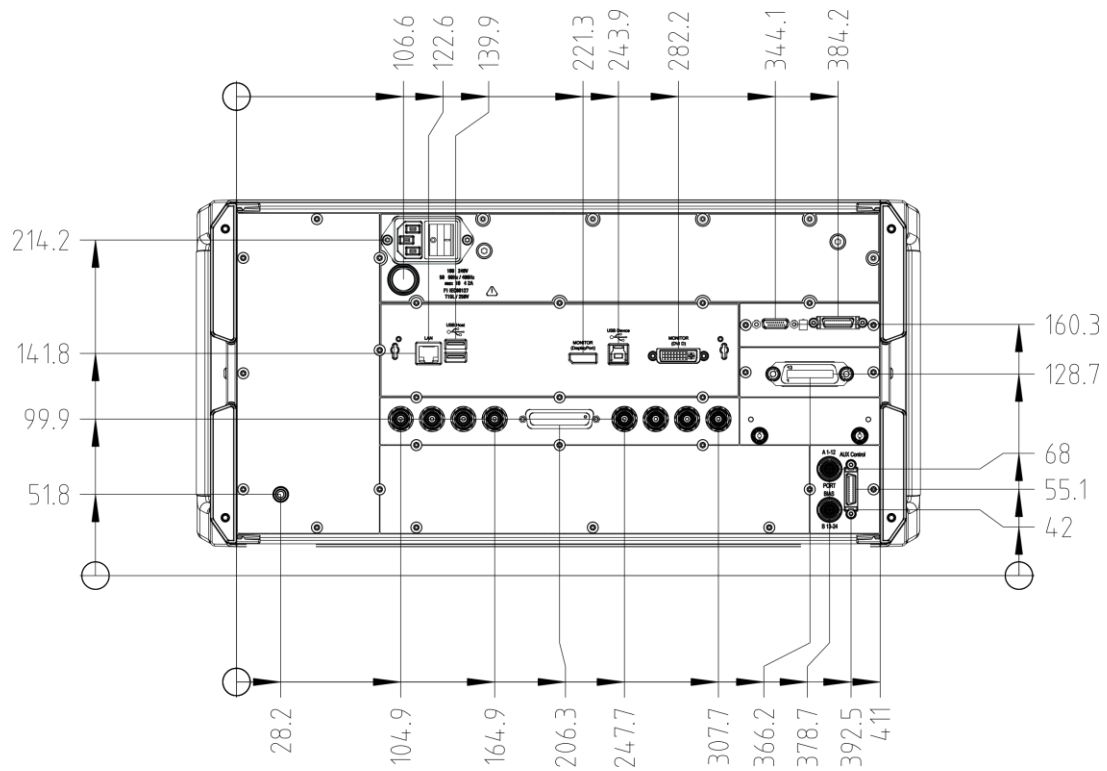
Rear view of the R&S®ZNBT8, R&S®ZNBT20, R&S®ZNBT26 and R&S®ZNBT40
