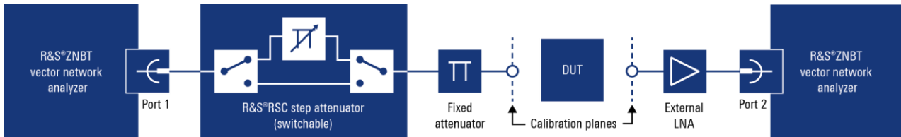
Recommended setup for R&S®ZNBT-K30 noise figure measurements
