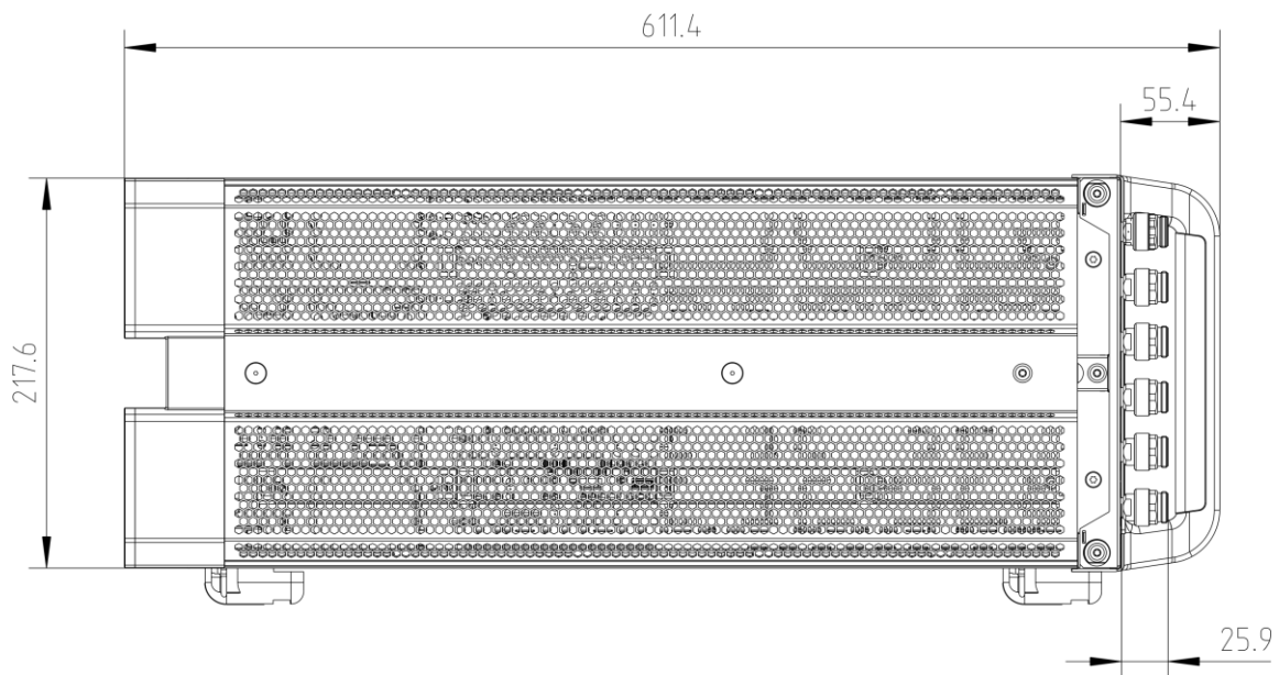
Side view of the R&S®ZNB T20, R&S®ZNB T26 and R&S®ZNB T40
