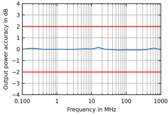
Measured output power accuracy in dB versus frequency for the R&S®ZNB20
