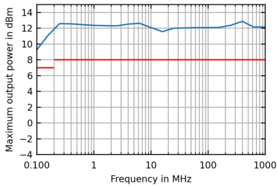
Measured maximum output power in dBm versus frequency for the R&S®ZNB26 and R&S®ZNB40
