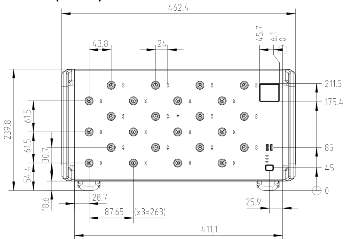
Front view of the R&S®ZNBT8
