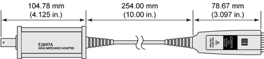
Figure 2 E2697A Dimensions
