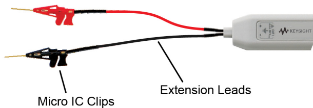
Figure 12 Extension Leads on Probe
