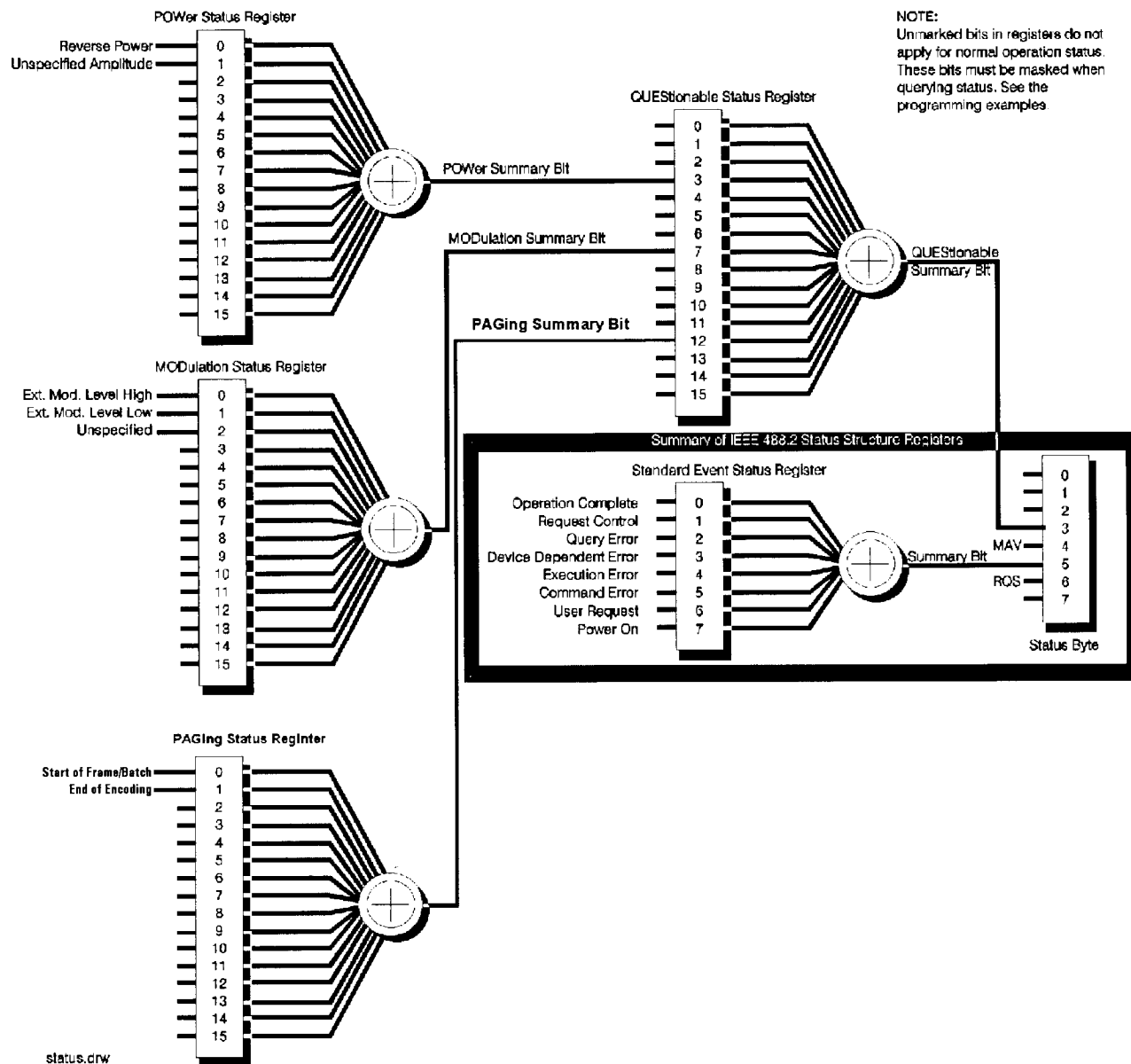
Figure 2-1. 8648 Status Register Model
