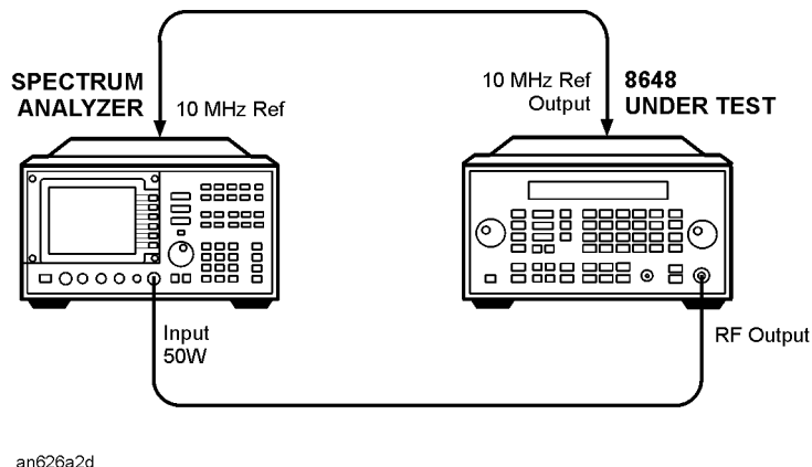
Figure 8-13. Harmonics Equipment Setup
