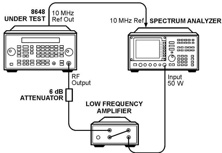
Figure 7-28. HF Power Level Accuracy Test Setup for Power Levels of < -70 dBm and \leq 1300 MHz
