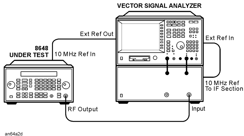
Figure 7-33. FSK Deviation Test Setup
