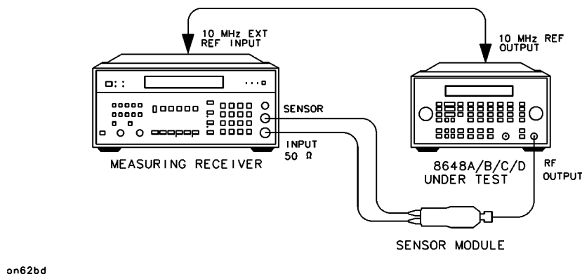
Figure 8-16. Equipment Setup for 8648A and 8648B/C/D \leq 1300 MHz
