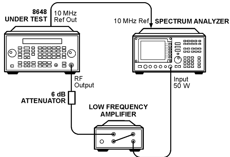
Figure 8-25. HF Power Level Accuracy Test Setup (Power Levels < -70 and \geq 1300 dBm)
