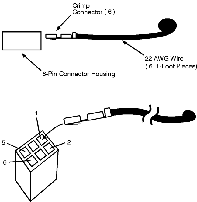
Figure 7-1. J31 Test Point Extender
