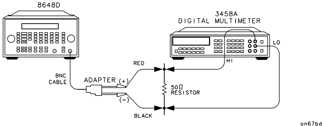
Figure 9-2. 9 kHz RF Level Accuracy Equipment Setup
