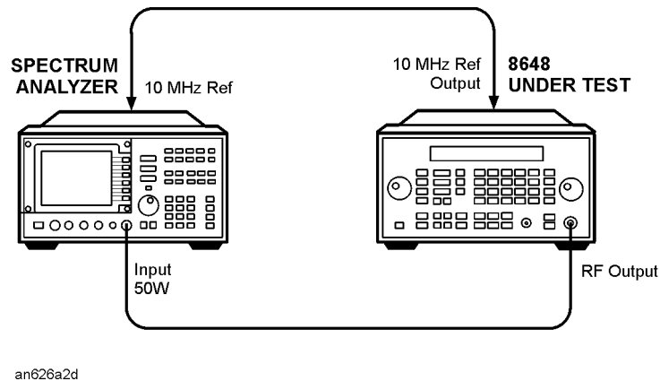
Figure 8-14. Spurious Equipment Setup
