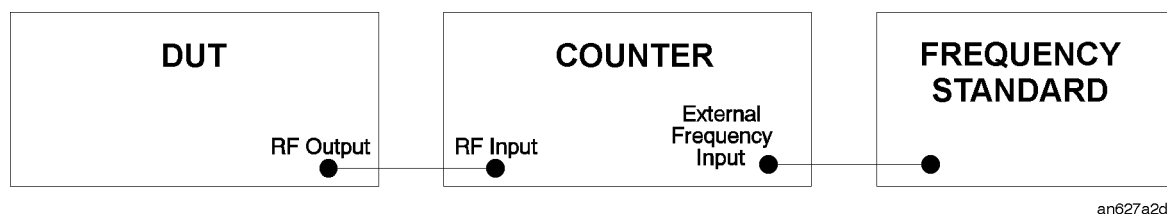
Figure 7-3. Internal Reference Oscillator Adjustment Setup
