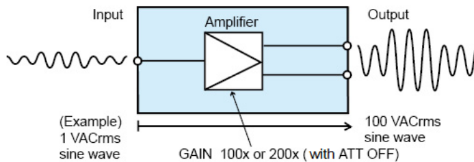
EXT-DC mode
