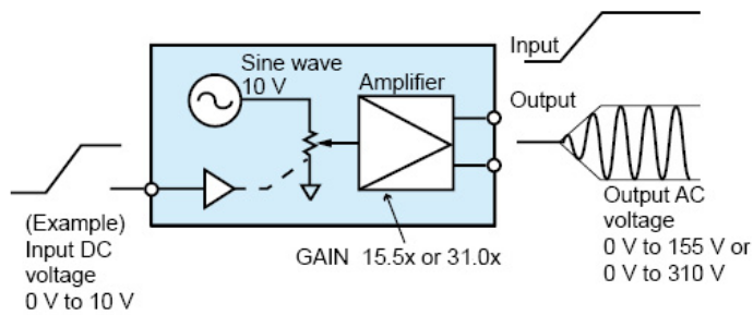
EXT-DC mode
